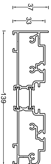
006.1901 Outerframe Bottom
